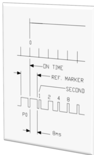
Figure 4 – 8 ms reference marker shows the start of the IRIG-B frame. Sourced from IRIG Standard 200-04
