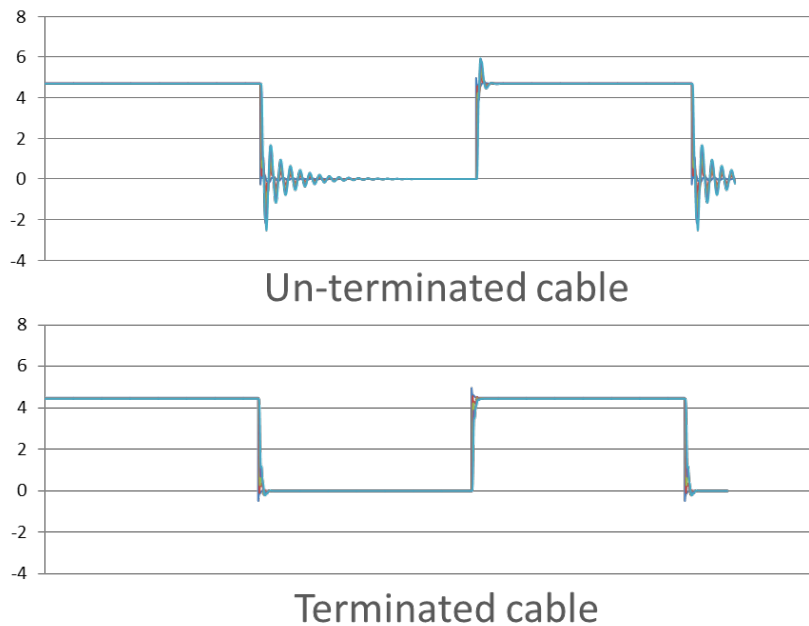
Figure 8 – Un Terminated line vs a Terminate Line
