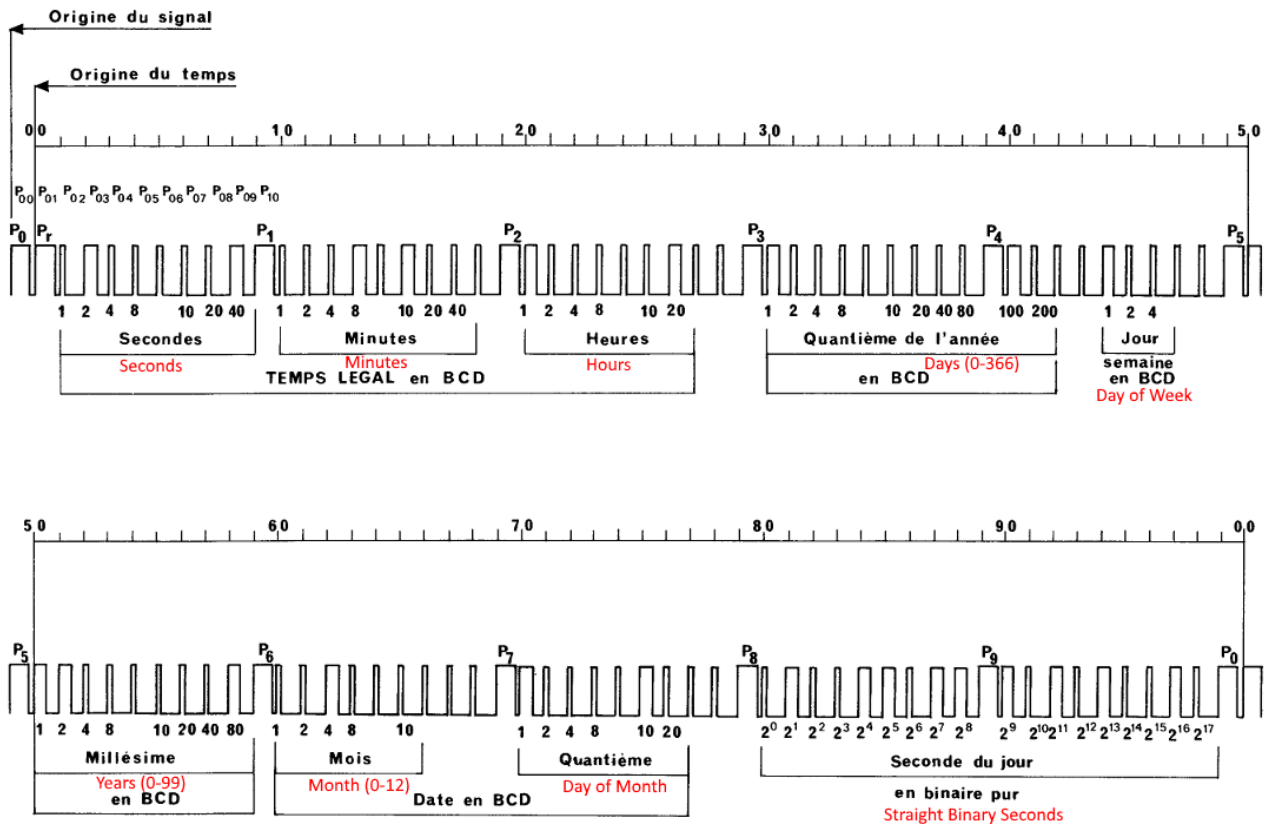
Figure 6 – IRIG-B code with AFNOR enabled. Sourced from AFNOR NFS 87-500 Standard.
