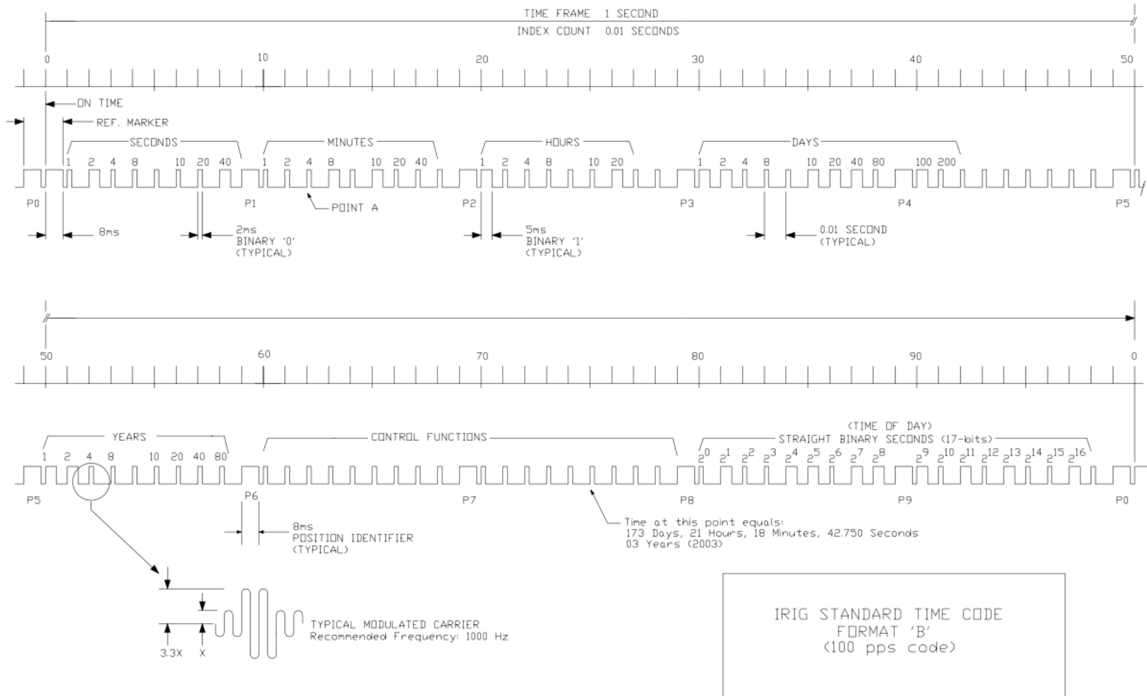
Figure 5 – Complete IRIG-B signal with data listed. Sourced from IRIG Standard 200-04
