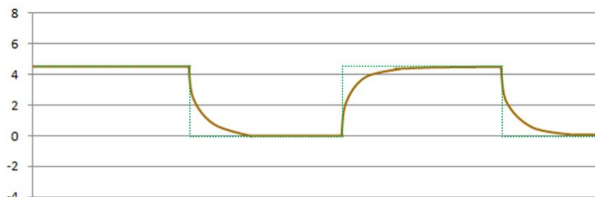
Figure 7 – Signal rounding caused by the capacitance of a coaxial cable
