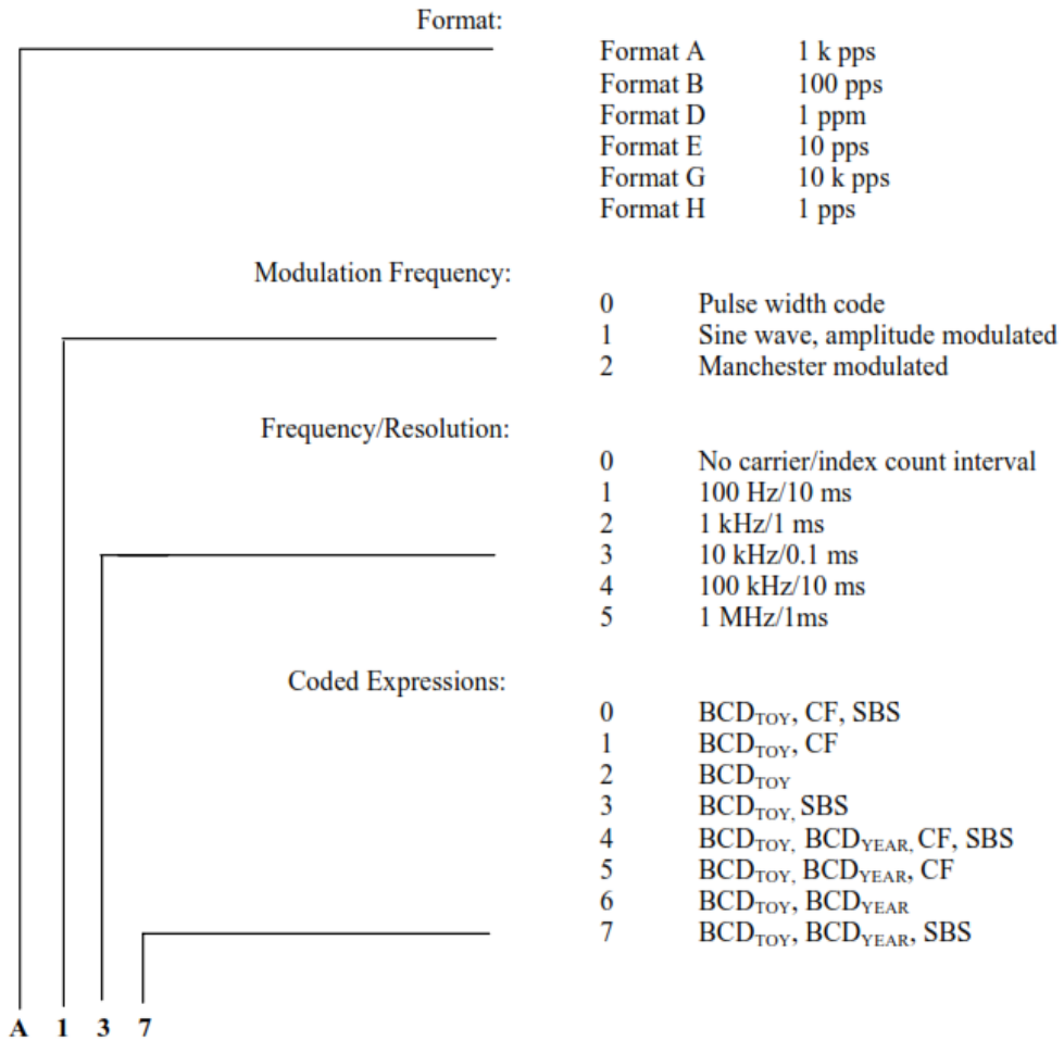
Figure 3 – IRIG Code Reference Guide sourced from IRIG Standard 200-04
