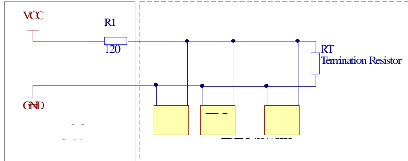
Figure 9 – Example implementation for a termination resistor at the end of an IRIG-B bus.
